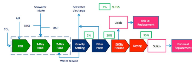
Figure 1. Technology process lineup for fishmeal and fish oil replacement products from algae.
