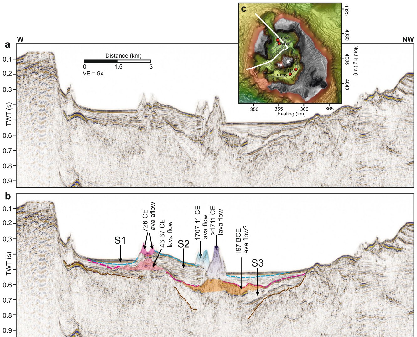
Extended Data Fig. 2 | Seismic profile across the northwestern flank of Kameni volcano and the northern caldera basin. a, b, Un-interpreted ( a ) and interpreted ( b ) version of a seismic profile crossing the western breach, the northwestern flank of the Kameni edifice and the northern caldera basin. c, Map of Santorini caldera showing the location of the seismic profile in ( a ) and ( b ).
