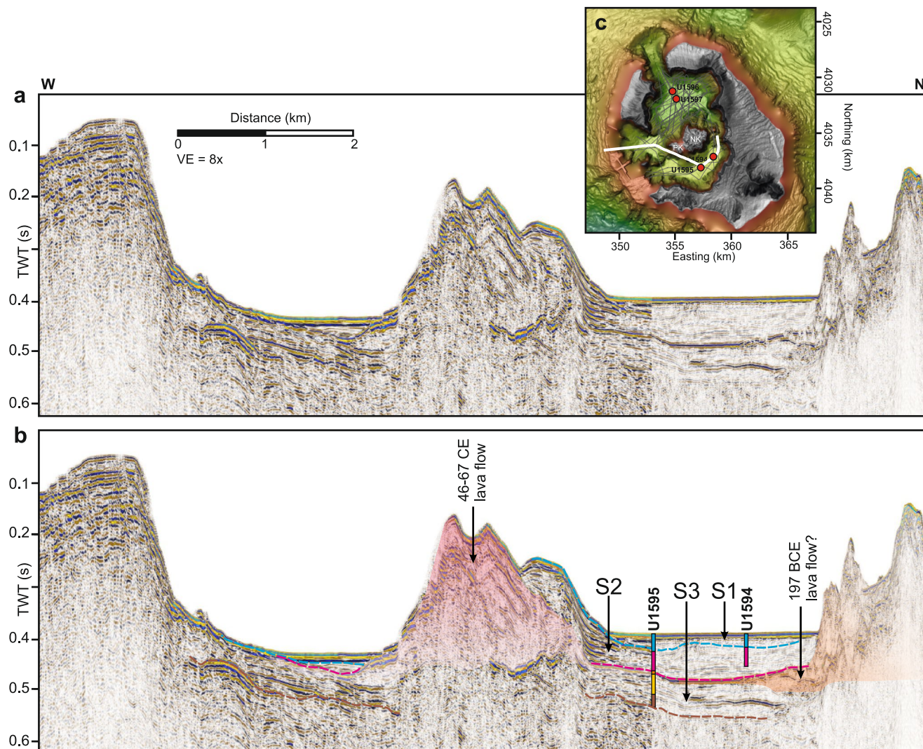
Extended Data Fig. 1 | Seismic profile across the western flank of Kameni volcano and the southern caldera basin. a, b, Un-interpreted (a) and interpreted (b) version of a seismic profile crossing the western breach, the western flank of the Kameni edifice and the southern caldera basin with Sites
